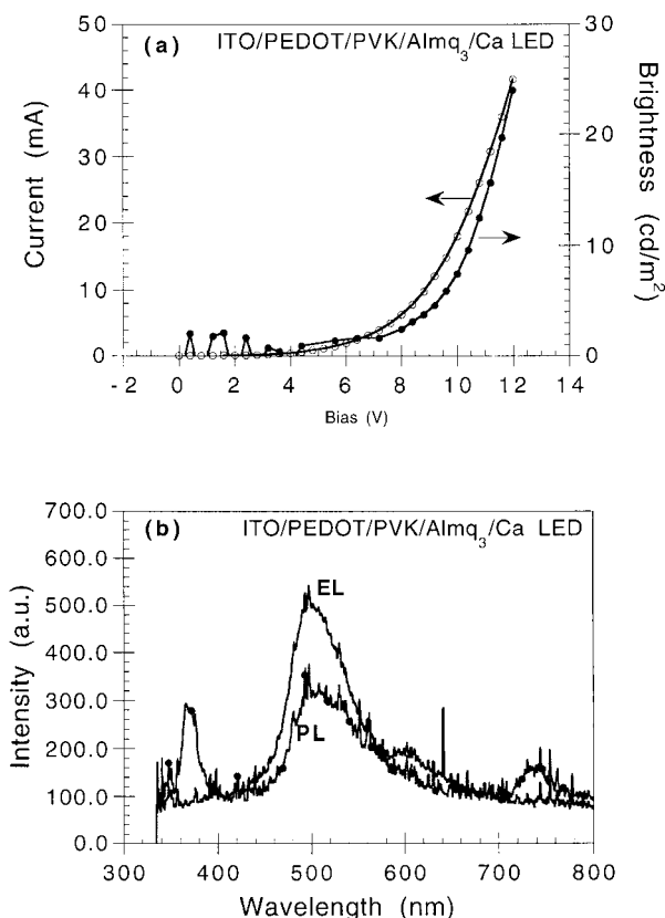
Fig. 3. a) The current-voltage and light-voltage ( I - V and L - V ) curves for the ITO/PEDOT/PVK/ \text{Almq}_3 /Ca LED. b) EL and PL emission spectra for the same device.
